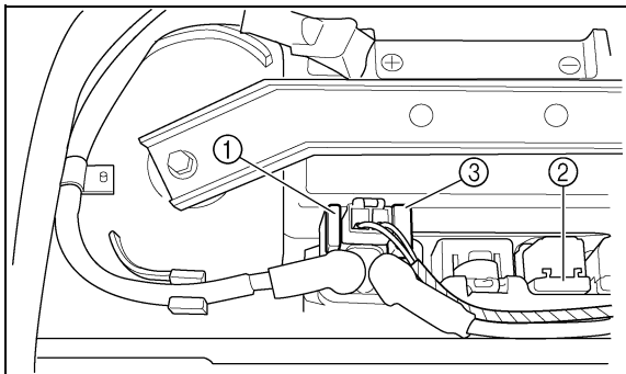
1. Main fuse 2. Four-wheel-drive fuse 3. Spare main fuse
