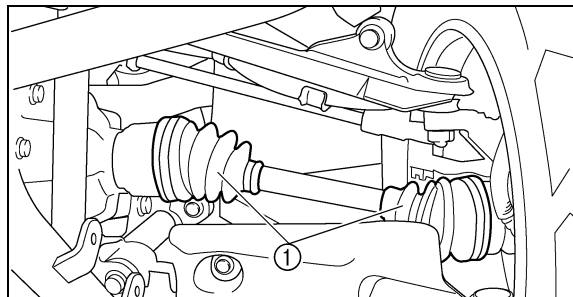
1. Axle boot (× 2)
