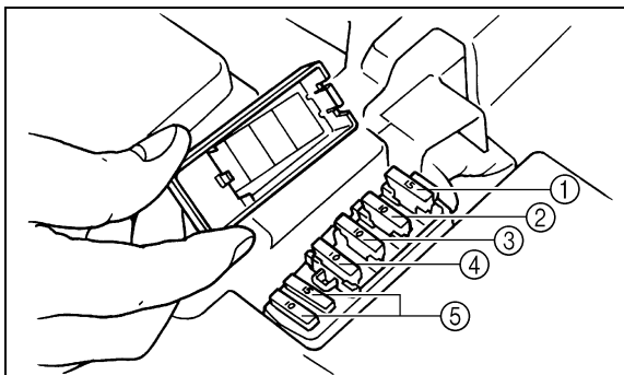
1. Headlight fuse 2. Ignition fuse 3. Auxiliary DC jack fuse 4. Carburetor warmer fuse 5. Spare fuse (× 2)
