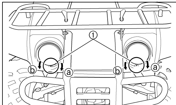
1. Headlight beam adjusting screw (× 2)
