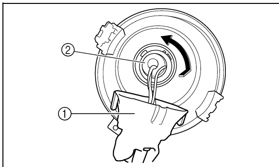
1. Headlight bulb holder cover 2. Headlight bulb holder
